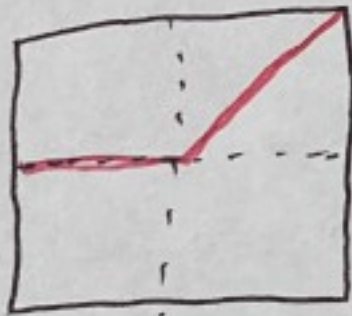
RELU
